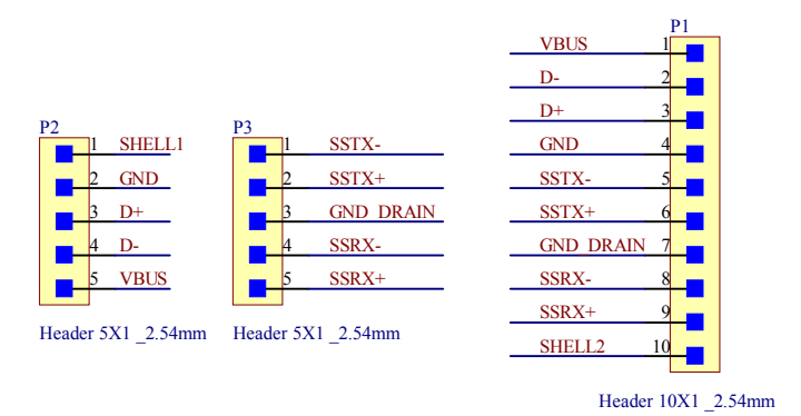
USB3-BF-BO-V1A Schematic Diagram
