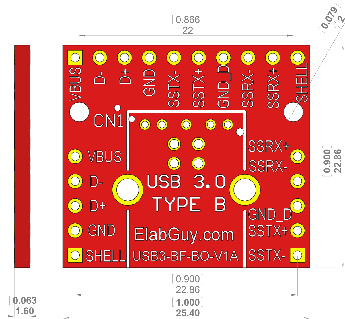
USB3-BF-BO-V1A PCB Outline Drawing
